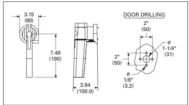
Figure 15. Pistol Handle — Type H
